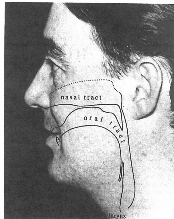
Figure 1.2 The vocal tract.
